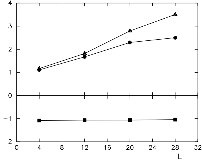
Fig.3. Ground-state energy per site E/L , on-site pairing correlation function P_0 and largest eigenvalue \lambda_0 of the reduced two-particle density matrix as a function of system size L for the Hubbard model with correlated hopping for t = 1 , \Delta t = 0.4 , U = -1 and n = 1.5 . Squares: E/L ; bullets: P_0 ; triangles: \lambda_0 . The lines are guides to the eye.
